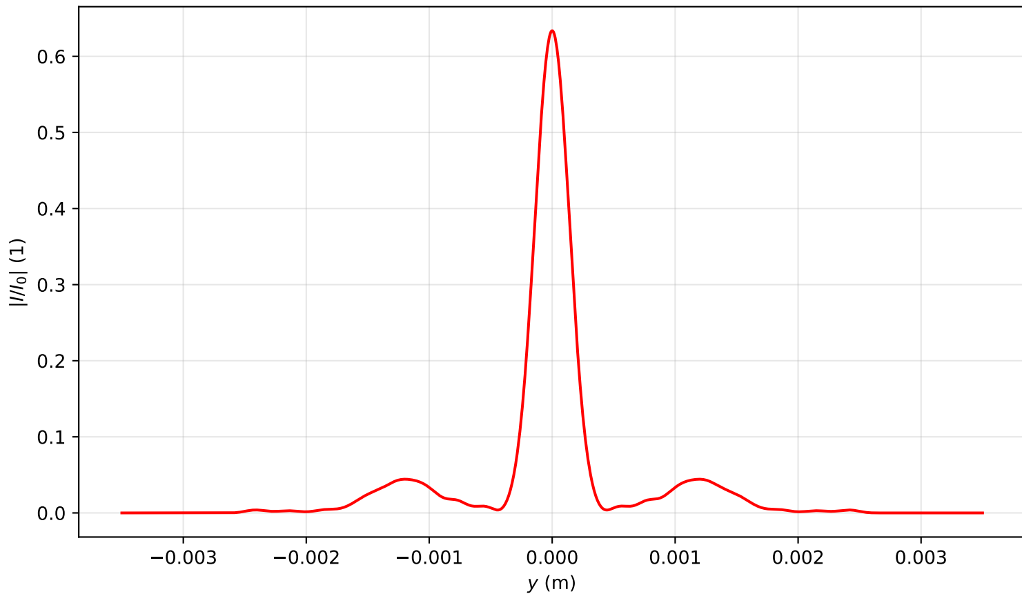
Intensity profile I(x=0, y, z=2.627)/I_0 , \text{Pin}=9.0\text{Pcr} , artificial time
